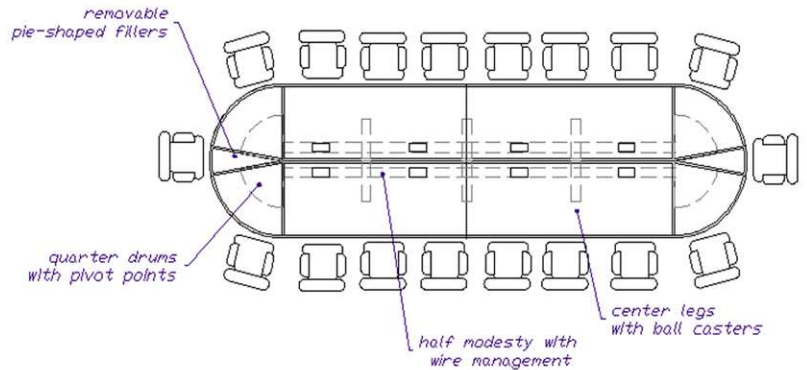
Plan View Of Video-Conferencing Table Closed
